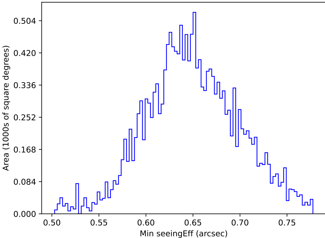
mw_roll_all_v3.3_10yrs WFD g band: Min seeingEff
