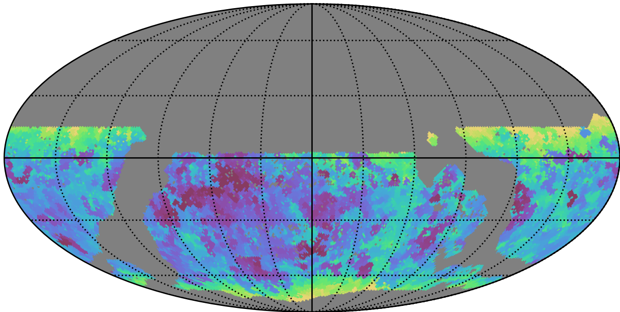
mw_roll_all_v3.3_10yrs WFD all bands: Min seeingEff
