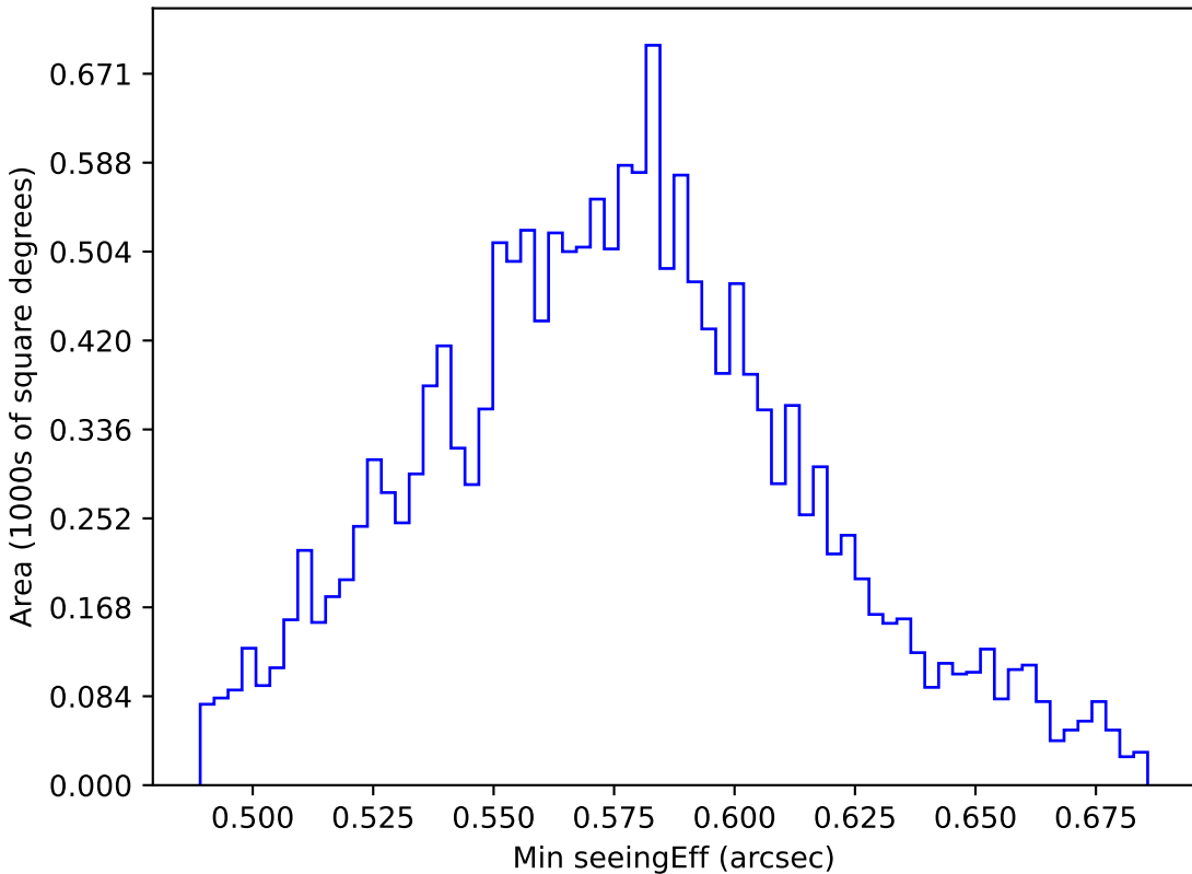
mw_roll_all_v3.3_10yrs WFD all bands: Min seeingEff
