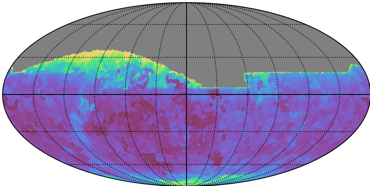
mw_roll_all_v3.3_10yrs All sky z band: Min seeingEff
