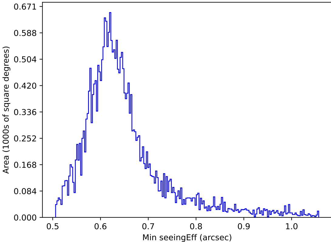
mw_roll_all_v3.3_10yrs All sky z band: Min seeingEff
