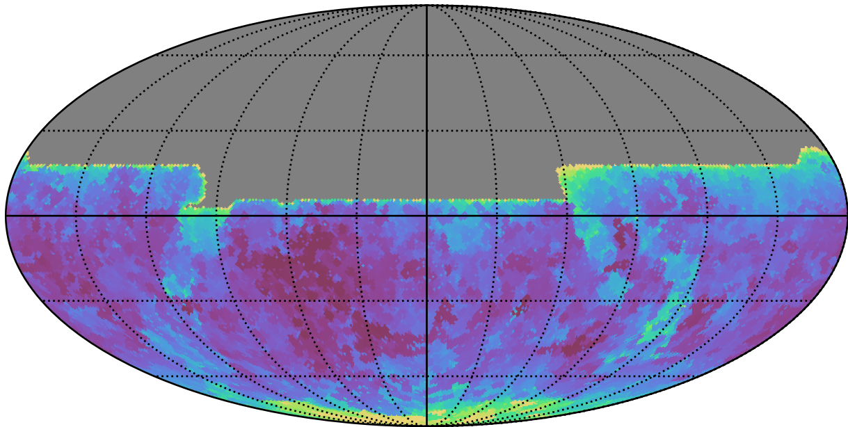
mw_roll_all_v3.3_10yrs All sky y band: Min seeingEff
