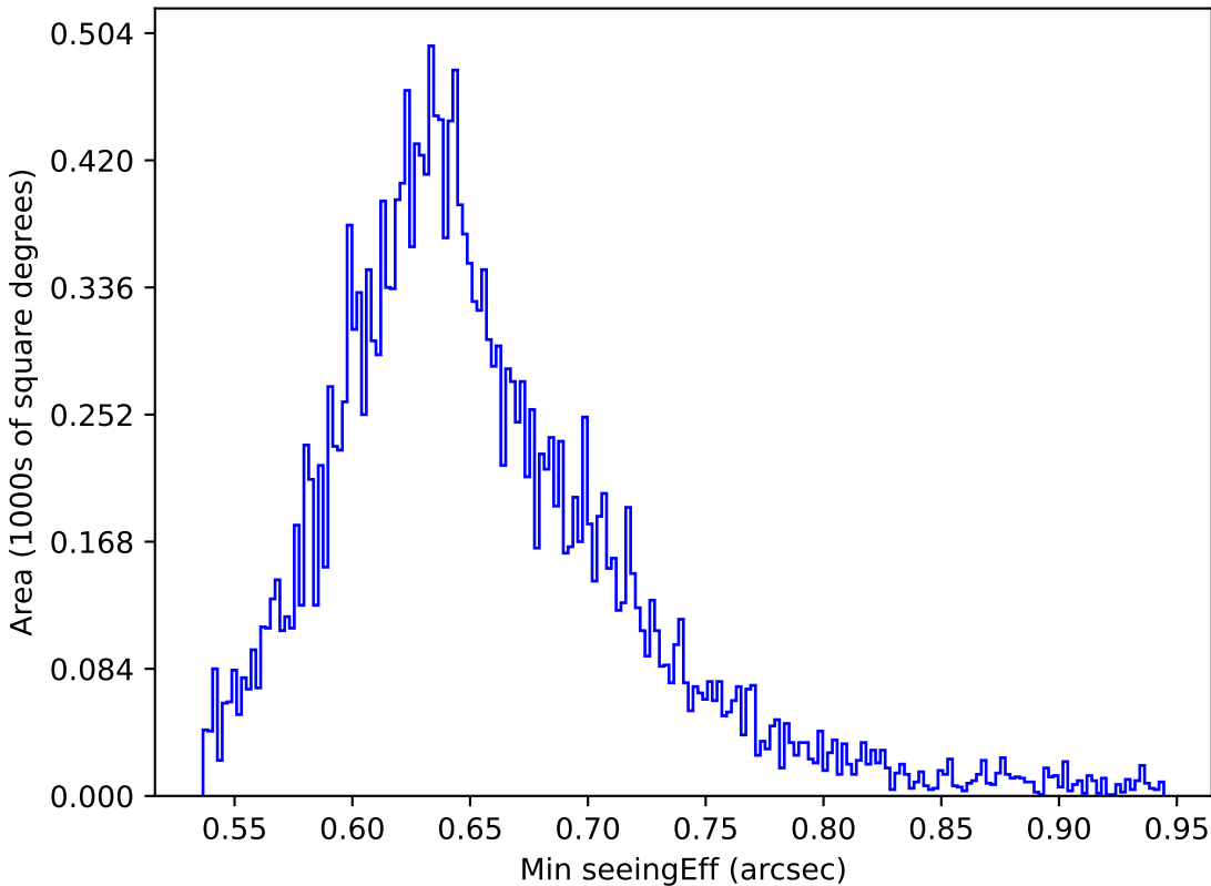
mw_roll_all_v3.3_10yrs All sky y band: Min seeingEff
