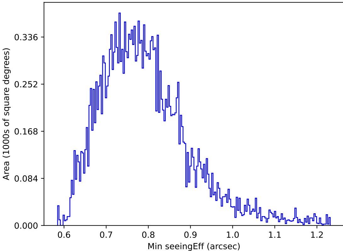
mw_roll_all_v3.3_10yrs All sky u band: Min seeingEff
