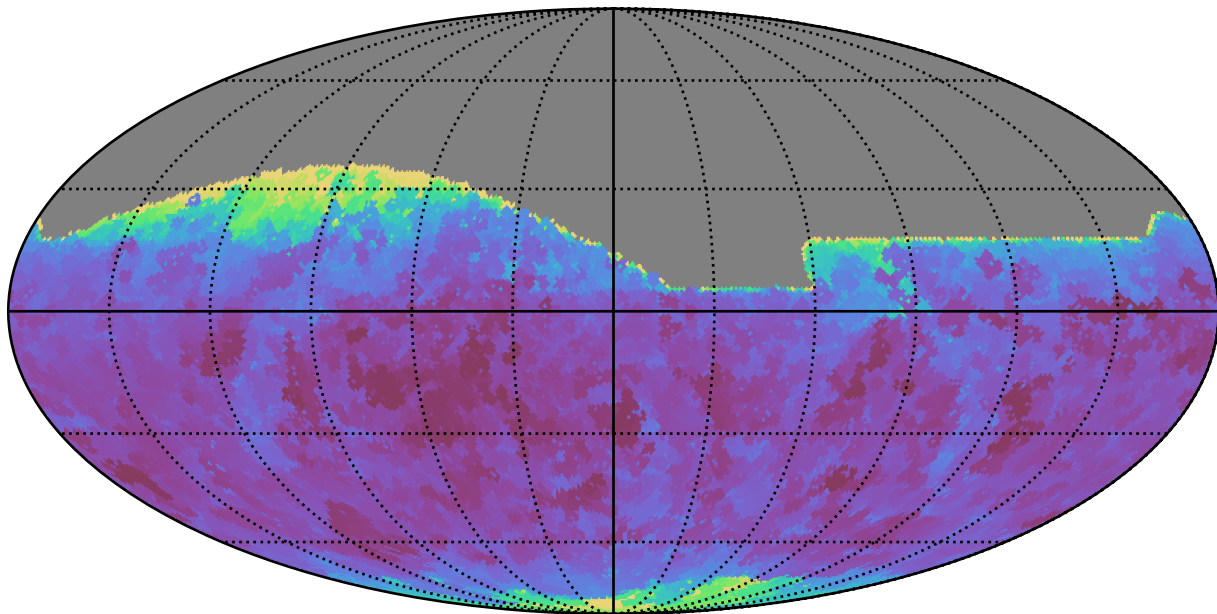
mw_roll_all_v3.3_10yrs All sky r band: Min seeingEff
