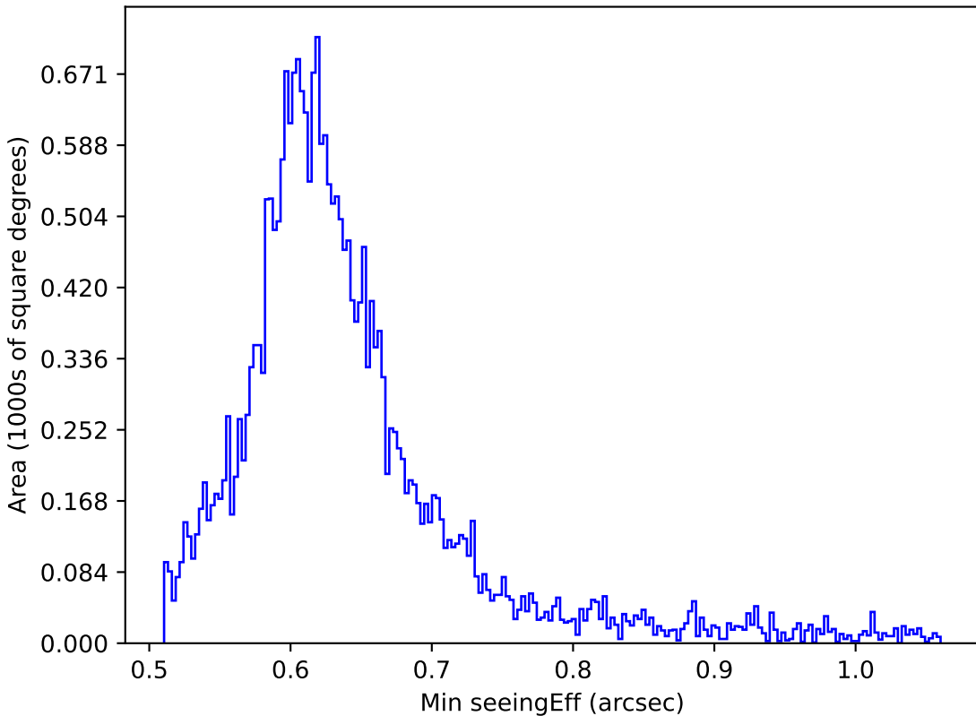
mw_roll_all_v3.3_10yrs All sky r band: Min seeingEff
