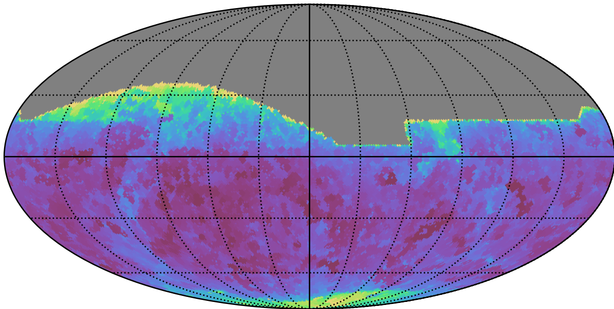
mw_roll_all_v3.3_10yrs All sky i band: Min seeingEff
