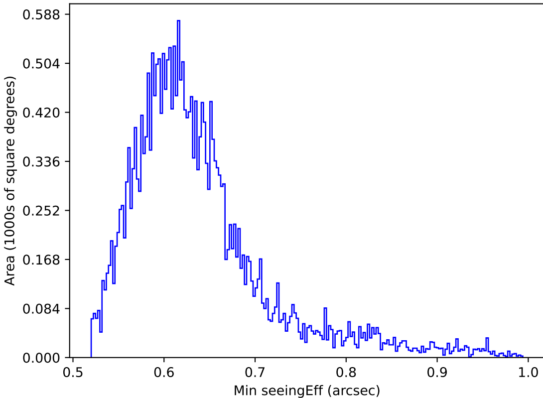
mw_roll_all_v3.3_10yrs All sky i band: Min seeingEff
