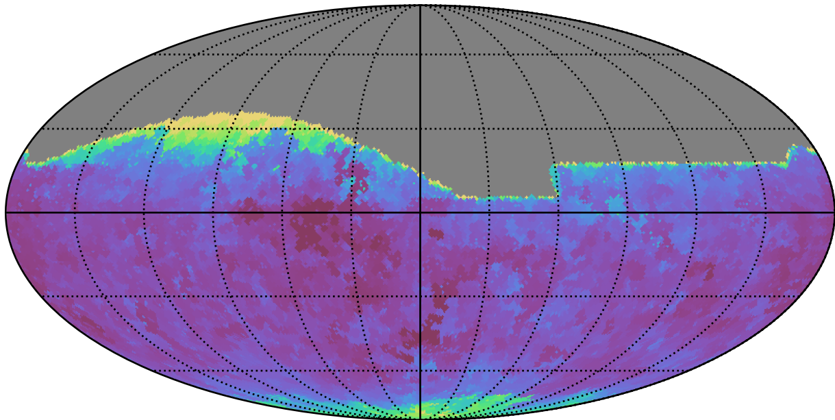
mw_roll_all_v3.3_10yrs All sky g band: Min seeingEff
