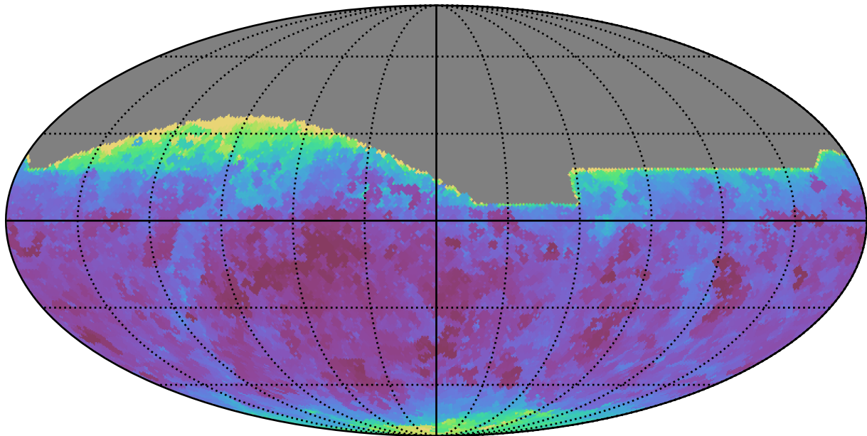
mw_roll_all_v3.3_10yrs All sky all bands: Min seeingEff
