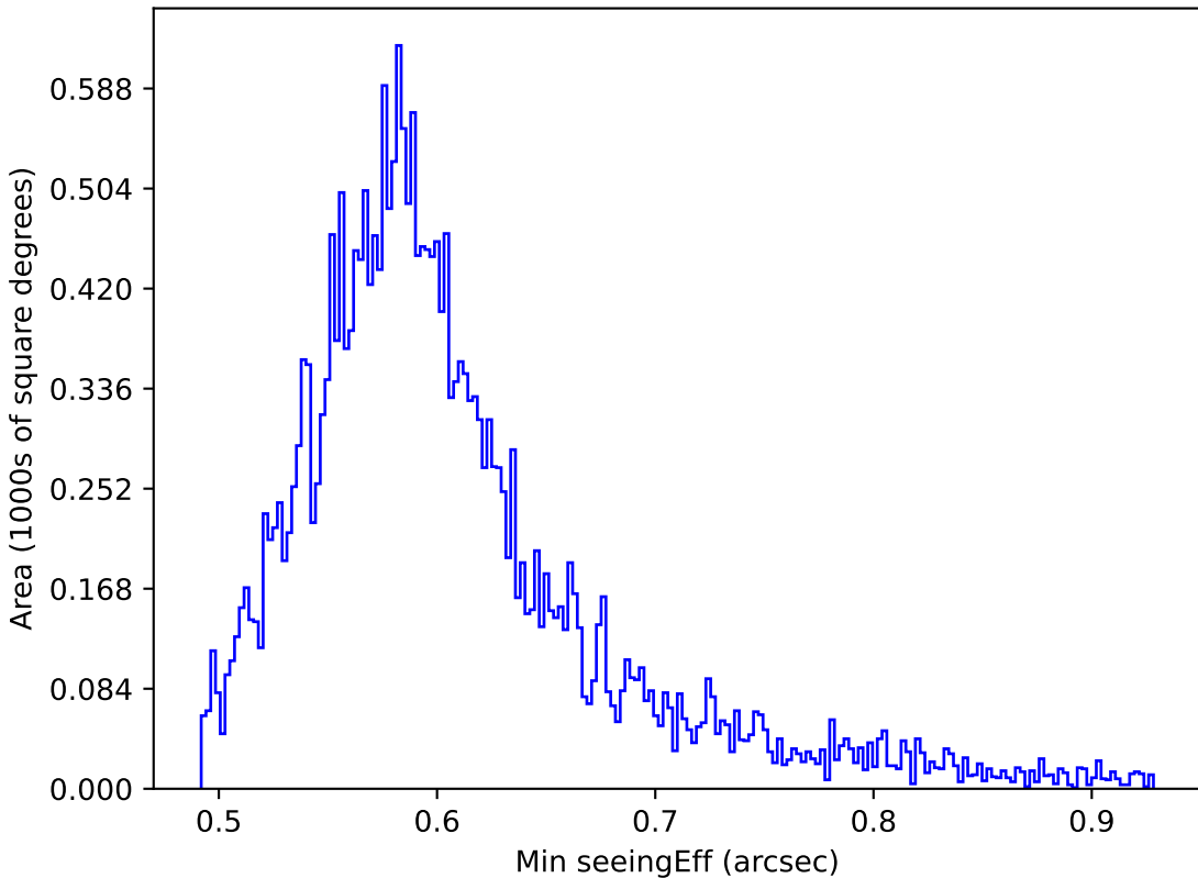
mw_roll_all_v3.3_10yrs All sky all bands: Min seeingEff
