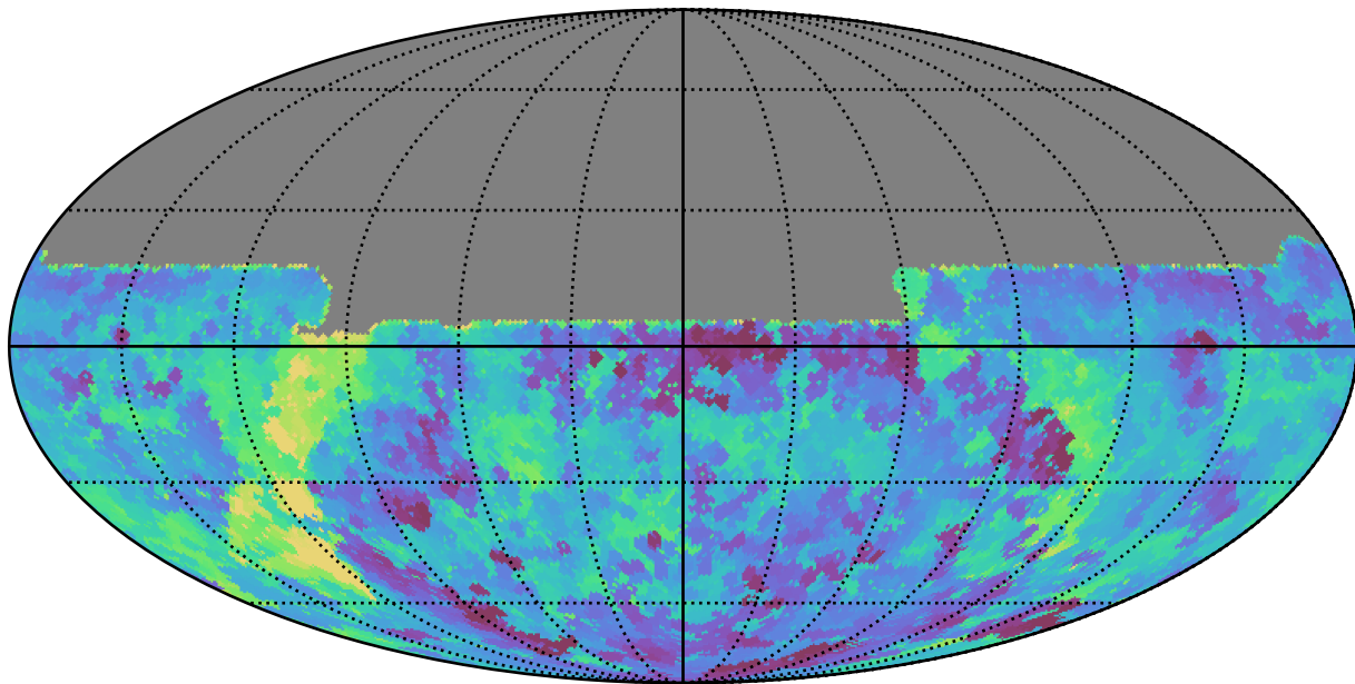
mw_roll_all_v3.3_10yrs All sky u band: Min saturation_mag
