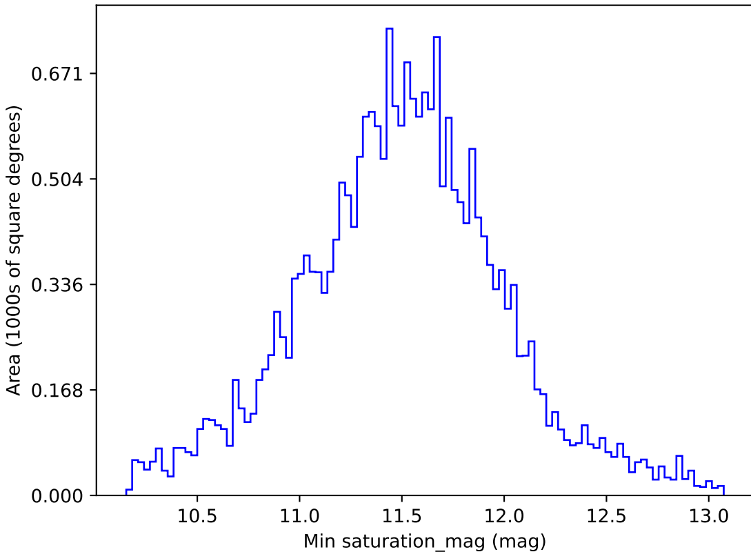
mw_roll_all_v3.3_10yrs All sky u band: Min saturation_mag
