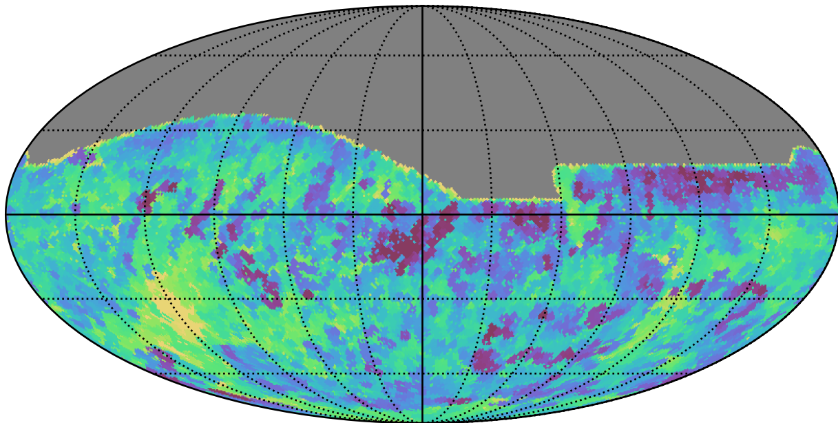
mw_roll_all_v3.3_10yrs All sky r band: Min saturation_mag
