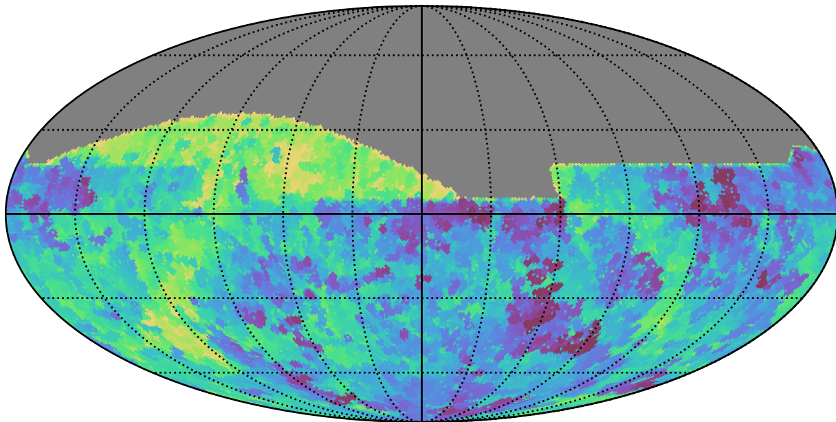
mw_roll_all_v3.3_10yrs All sky all bands: Min saturation_mag
