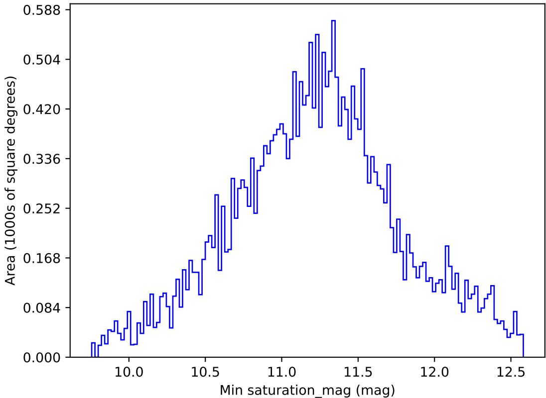
mw_roll_all_v3.3_10yrs All sky all bands: Min saturation_mag
