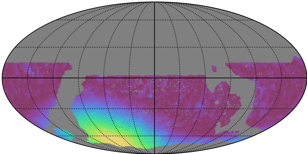
mw_roll_all_v3.3_10yrs WFD r band: Min moonDistance
