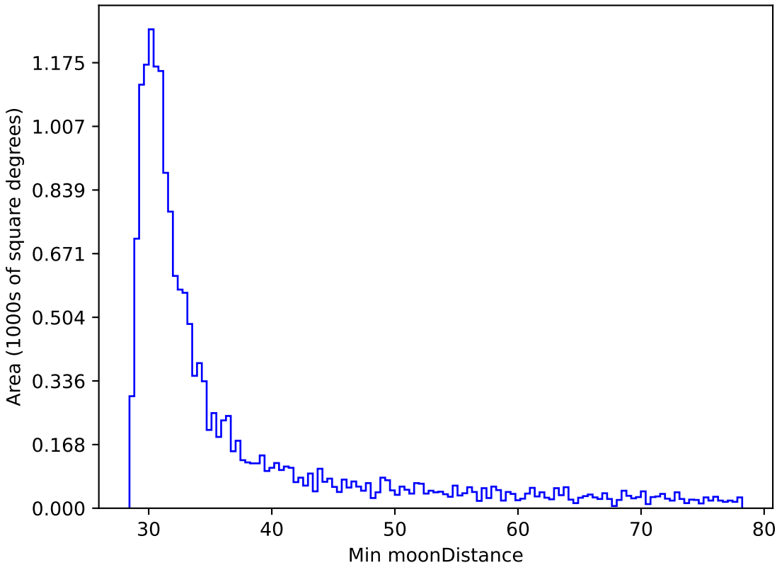
mw_roll_all_v3.3_10yrs WFD r band: Min moonDistance
