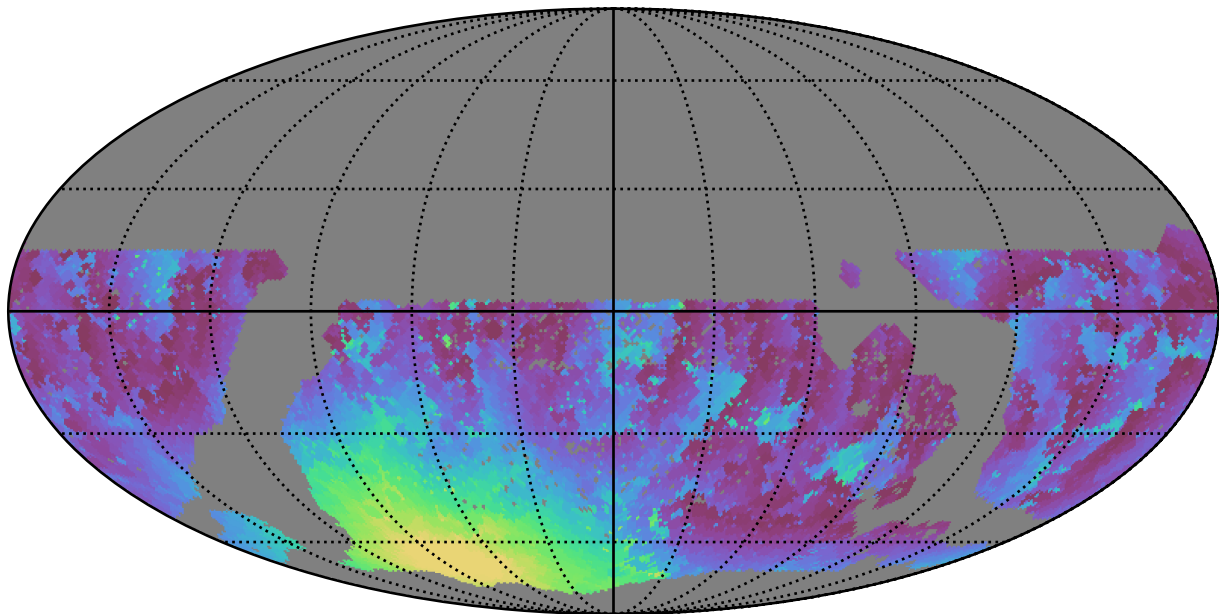
mw_roll_all_v3.3_10yrs WFD g band: Min moonDistance
