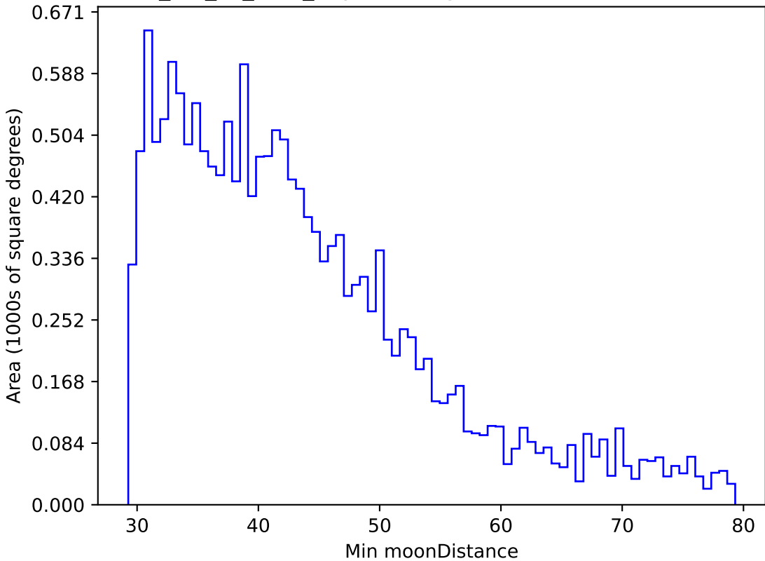
mw_roll_all_v3.3_10yrs WFD g band: Min moonDistance
