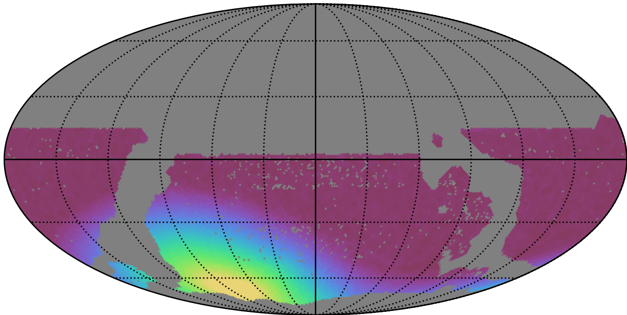
mw_roll_all_v3.3_10yrs WFD all bands: Min moonDistance
