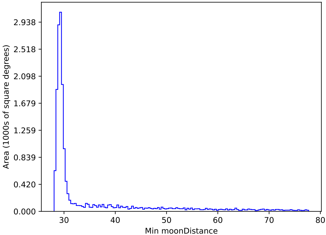
mw_roll_all_v3.3_10yrs WFD all bands: Min moonDistance
