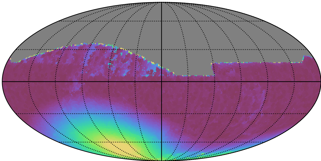
mw_roll_all_v3.3_10yrs All sky z band: Min moonDistance
