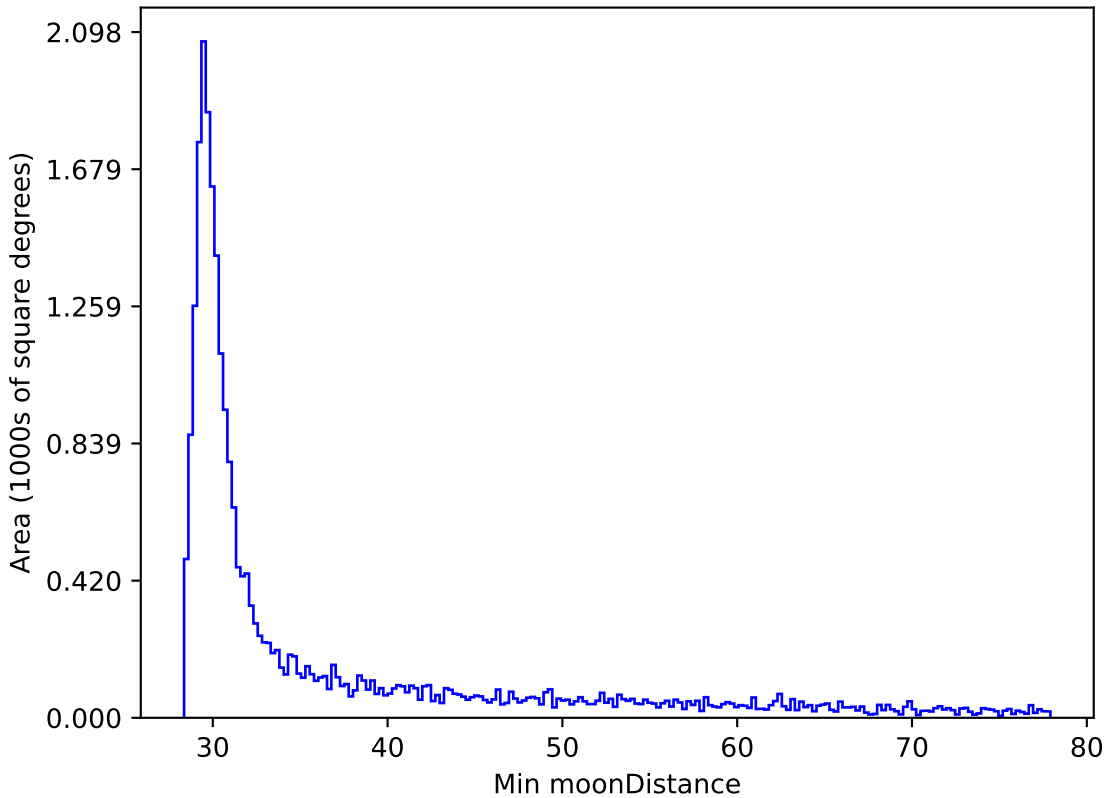
mw_roll_all_v3.3_10yrs All sky z band: Min moonDistance
