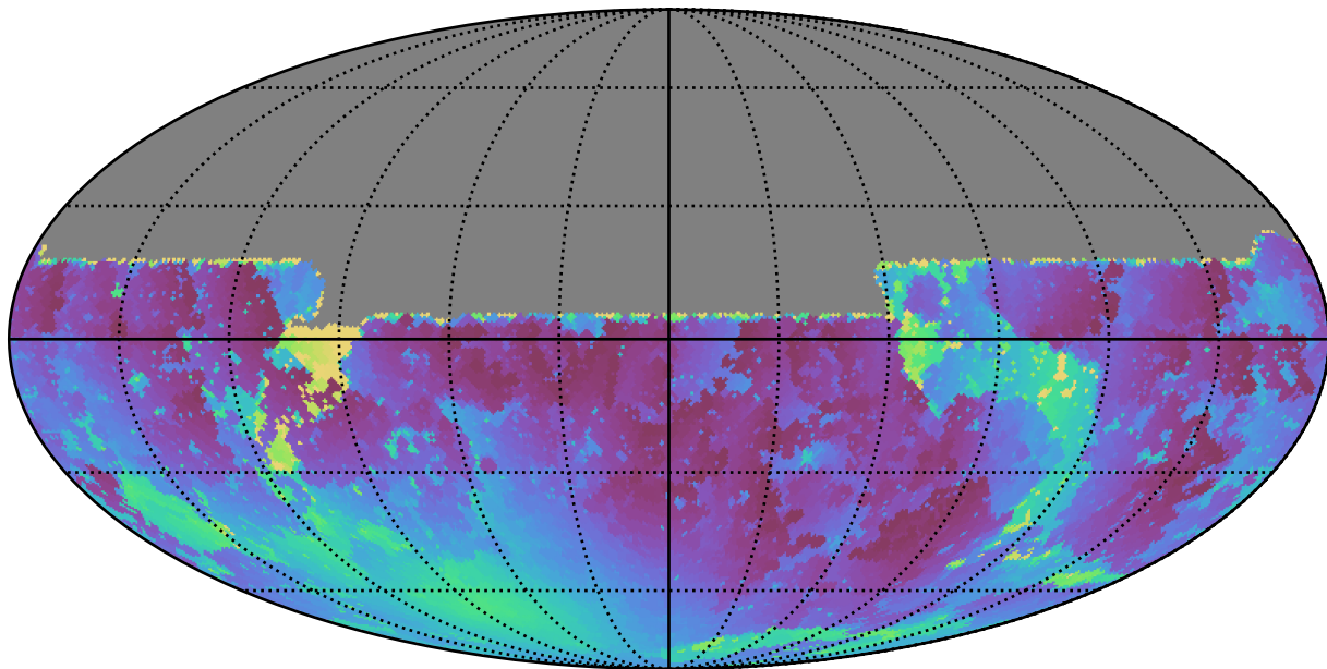
mw_roll_all_v3.3_10yrs All sky u band: Min moonDistance
