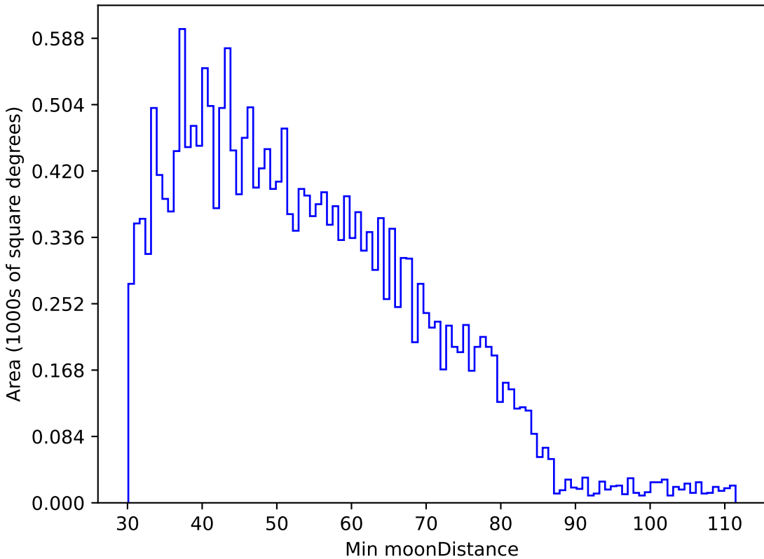
mw_roll_all_v3.3_10yrs All sky u band: Min moonDistance
