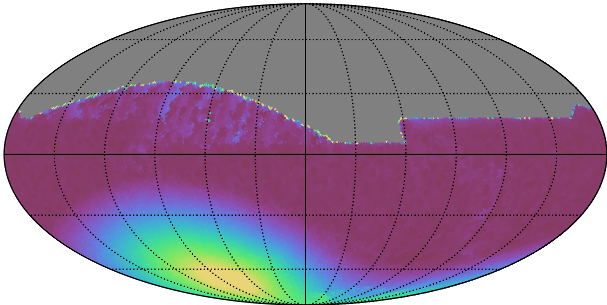
mw_roll_all_v3.3_10yrs All sky all bands: Min moonDistance
