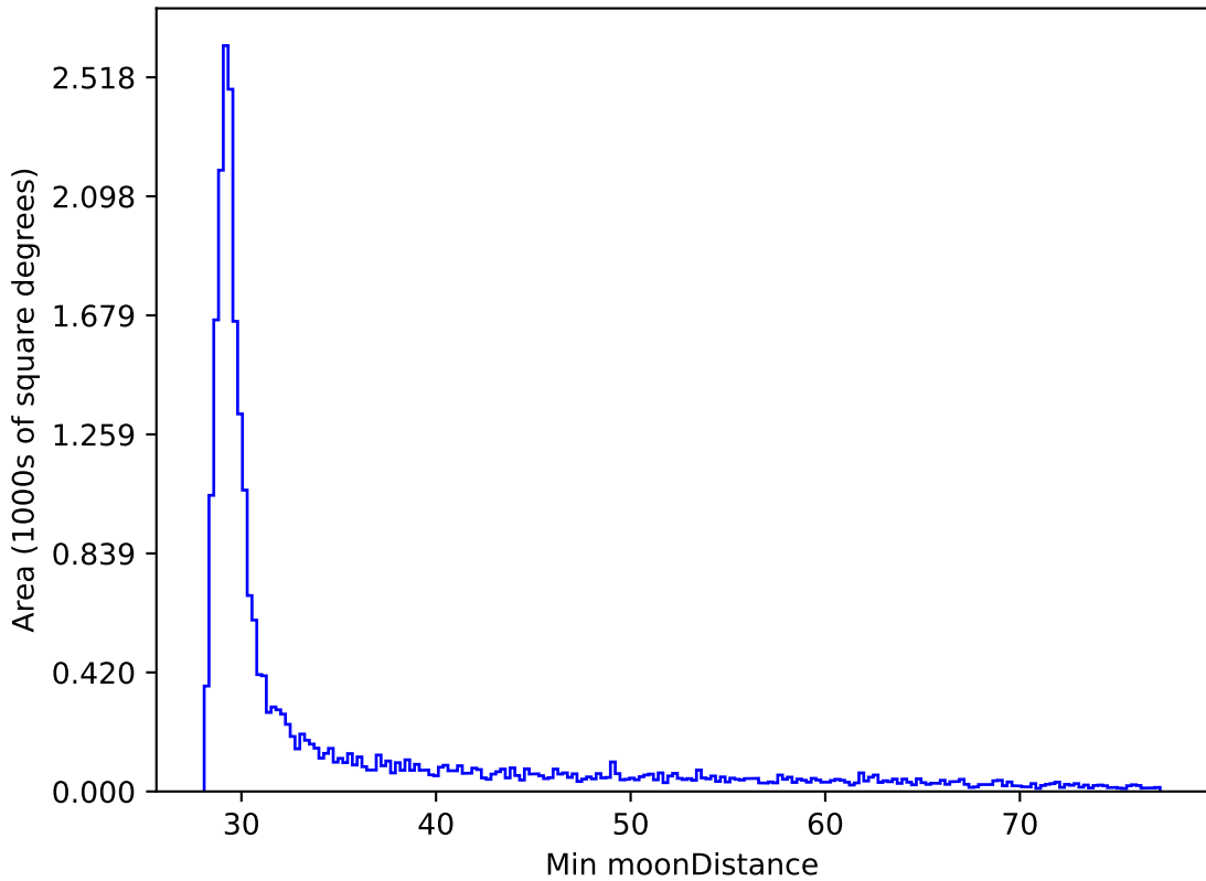
mw_roll_all_v3.3_10yrs All sky all bands: Min moonDistance
