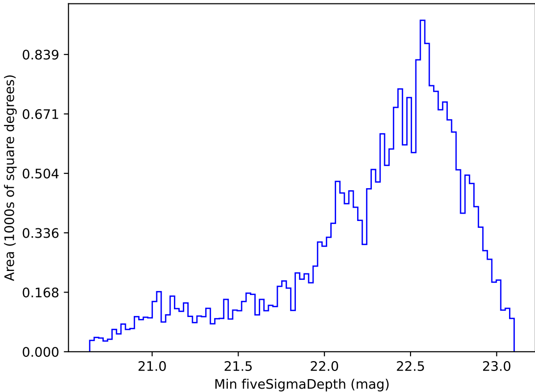
mw_roll_all_v3.3_10yrs Yr 1 z band: Min fiveSigmaDepth
