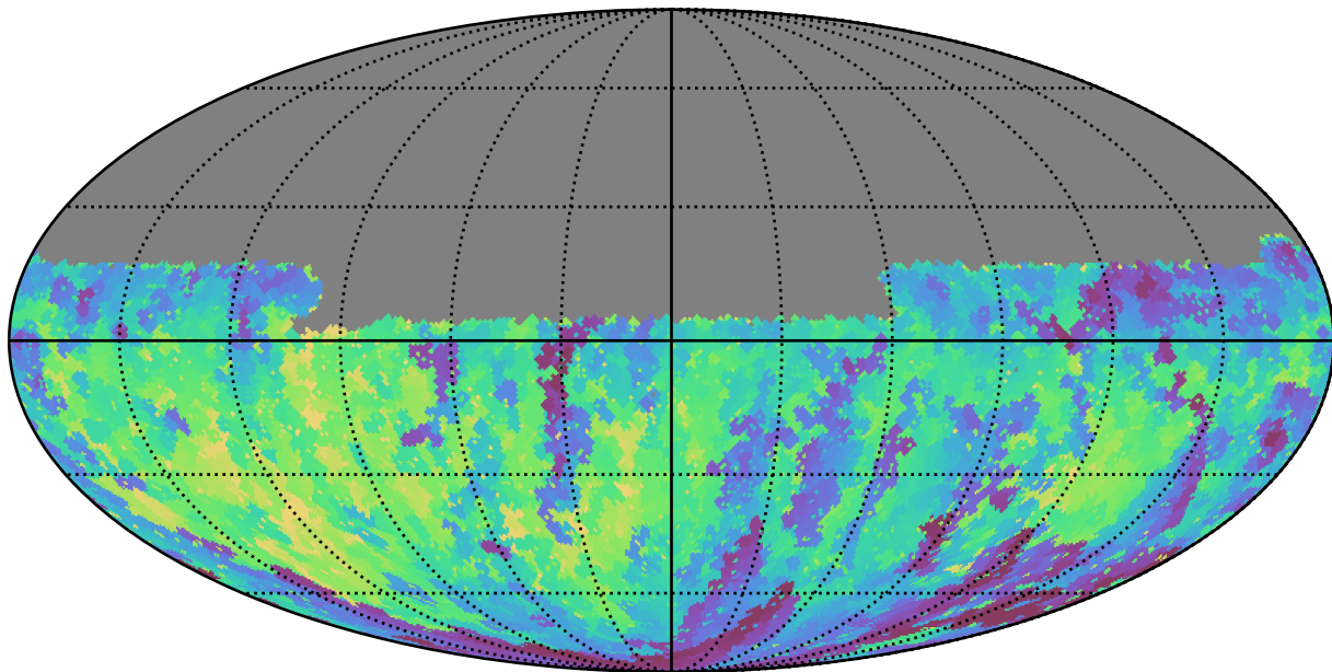
mw_roll_all_v3.3_10yrs Yr 1 u band: Min fiveSigmaDepth
