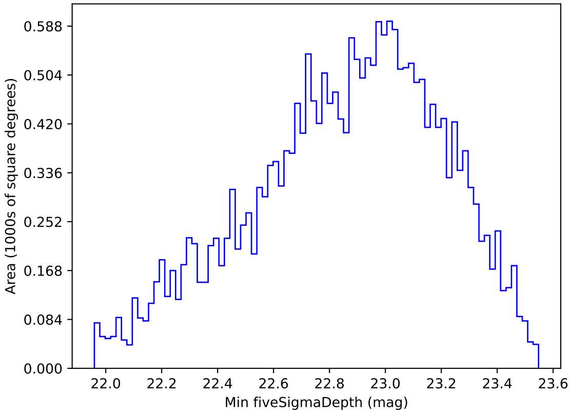
mw_roll_all_v3.3_10yrs Yr 1 u band: Min fiveSigmaDepth
