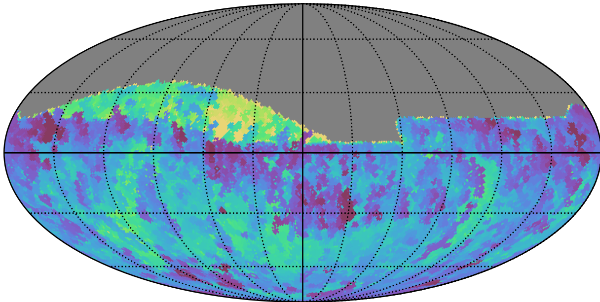
mw_roll_all_v3.3_10yrs Yr 1 all bands: Min fiveSigmaDepth
