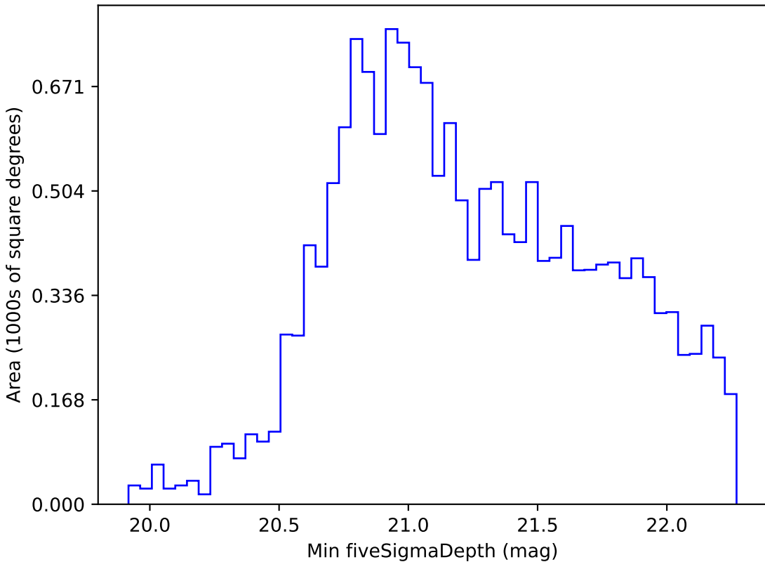
mw_roll_all_v3.3_10yrs WFD z band: Min fiveSigmaDepth
