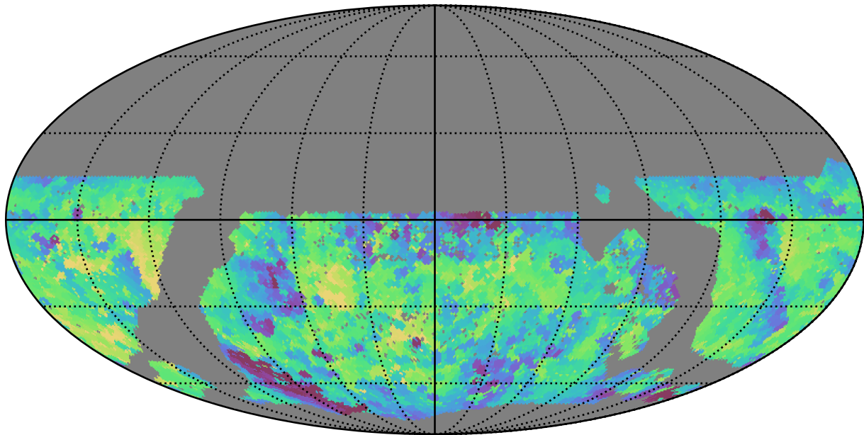
mw_roll_all_v3.3_10yrs WFD u band: Min fiveSigmaDepth
