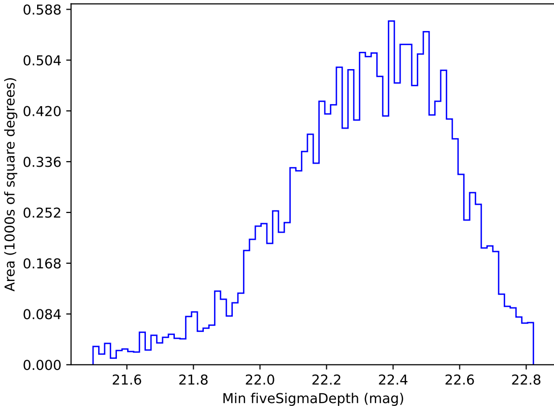
mw_roll_all_v3.3_10yrs WFD u band: Min fiveSigmaDepth
