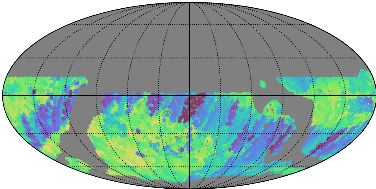
mw_roll_all_v3.3_10yrs WFD r band: Min fiveSigmaDepth
