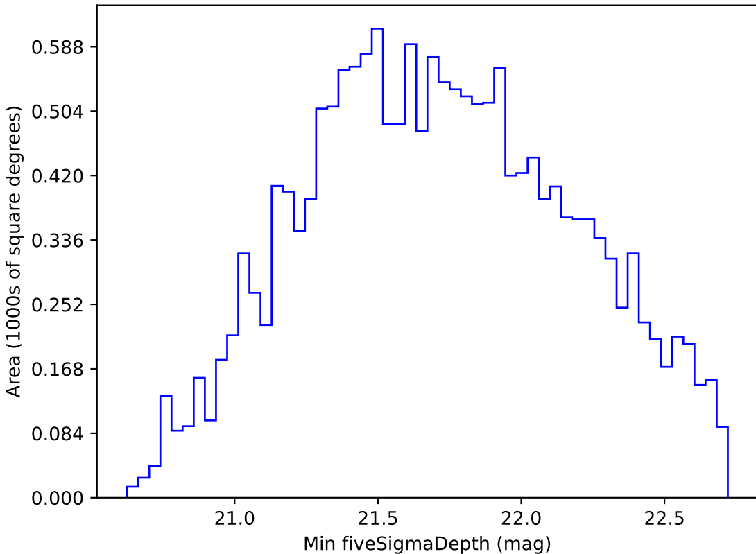
mw_roll_all_v3.3_10yrs WFD i band: Min fiveSigmaDepth
