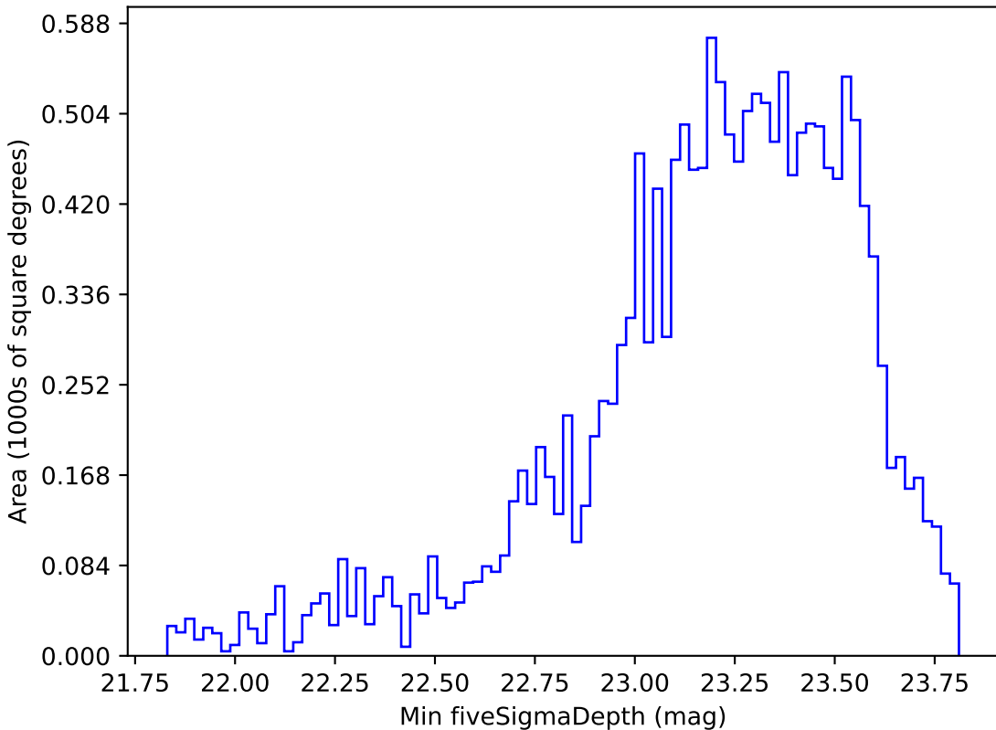
mw_roll_all_v3.3_10yrs WFD g band: Min fiveSigmaDepth
