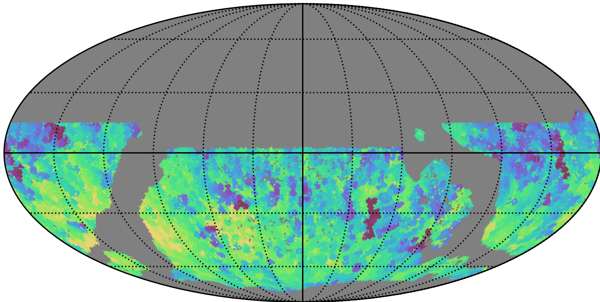
mw_roll_all_v3.3_10yrs WFD all bands: Min fiveSigmaDepth
