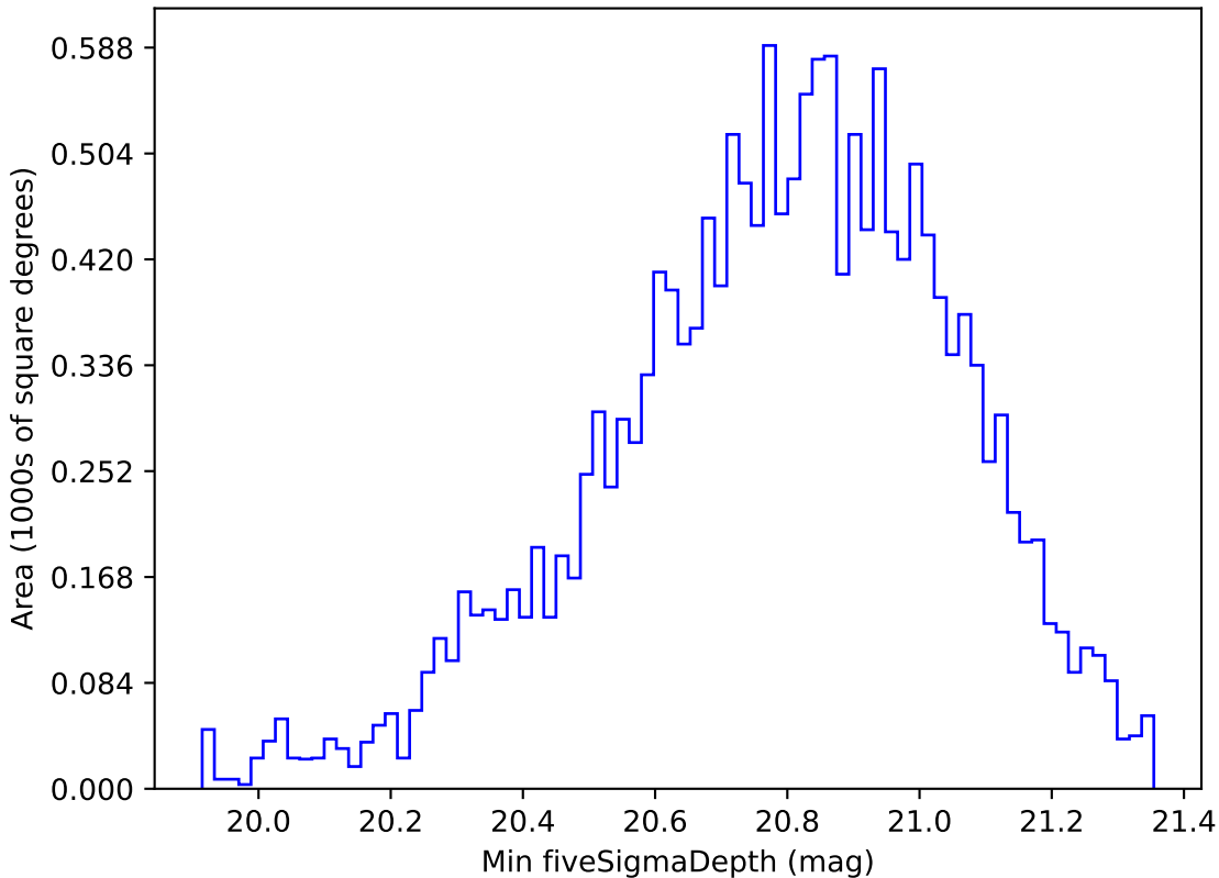
mw_roll_all_v3.3_10yrs WFD all bands: Min fiveSigmaDepth
