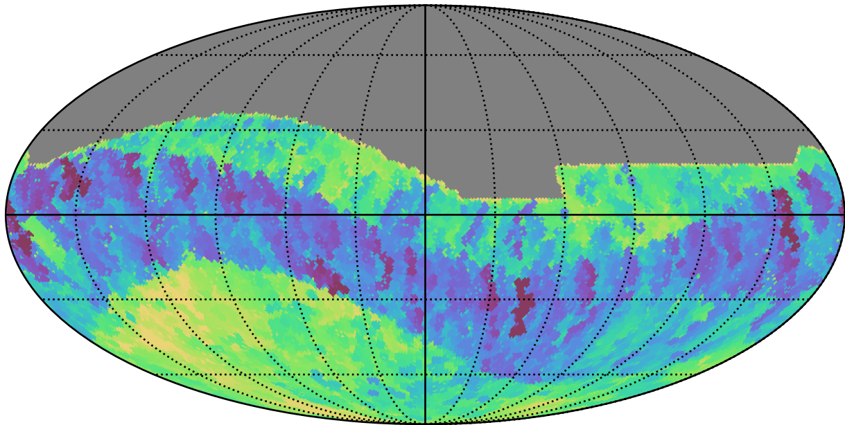
mw_roll_all_v3.3_10yrs All sky z band: Min fiveSigmaDepth
