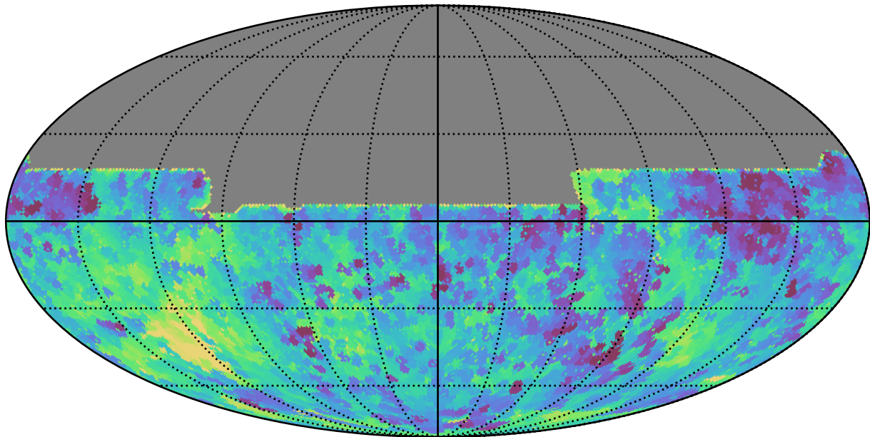
mw_roll_all_v3.3_10yrs All sky y band: Min fiveSigmaDepth
