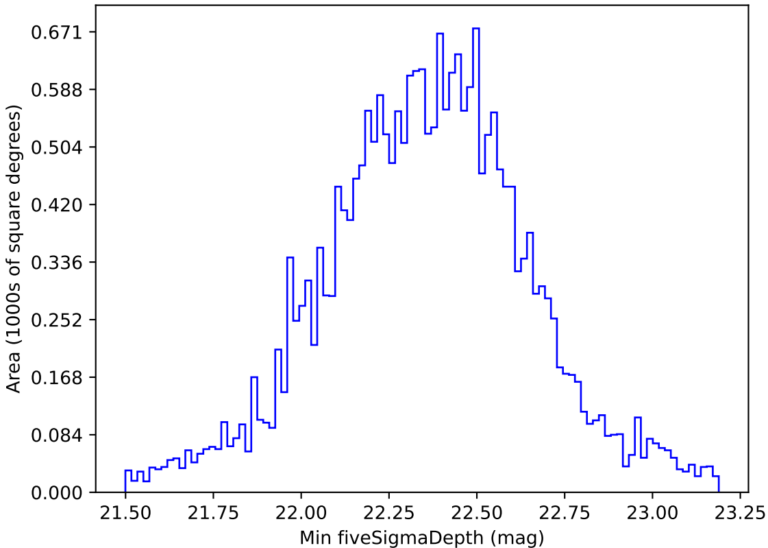
mw_roll_all_v3.3_10yrs All sky u band: Min fiveSigmaDepth
