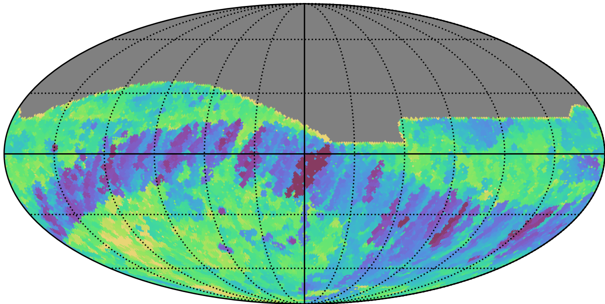
mw_roll_all_v3.3_10yrs All sky r band: Min fiveSigmaDepth
