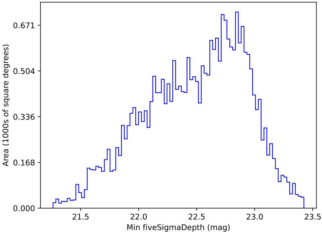
mw_roll_all_v3.3_10yrs All sky r band: Min fiveSigmaDepth
