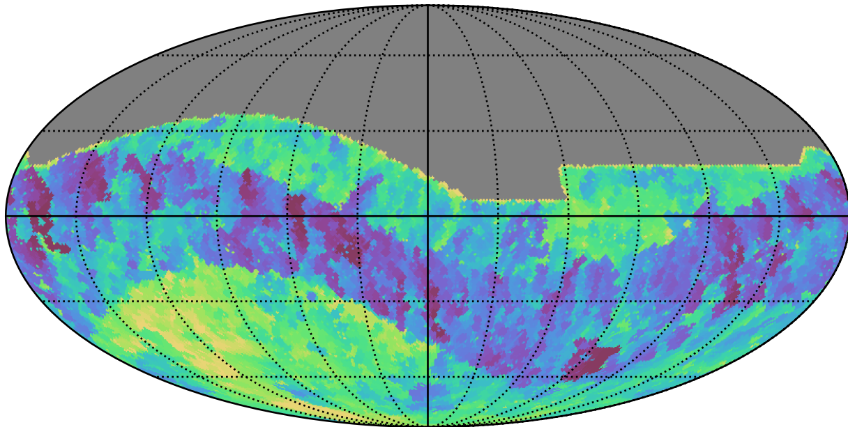
mw_roll_all_v3.3_10yrs All sky i band: Min fiveSigmaDepth
